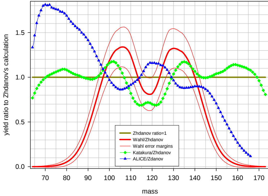
Benchmark B: ^{241}\text{Am} at 28 MeV, post neutron emission yield ratio to Zhdanov's data
